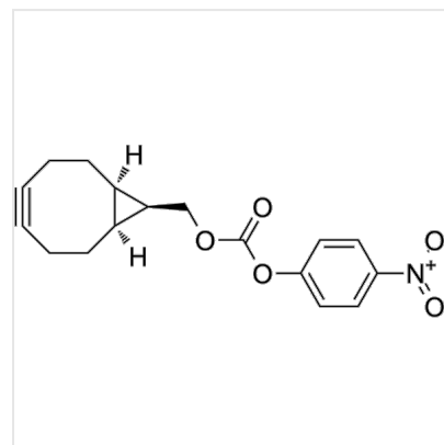
Structure endo-BCN-O-PNB, CAS 1263166-91-1
