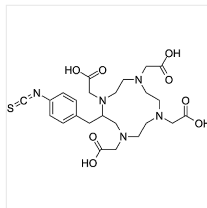
Structure p-SCN-Bn-DOTA, CAS 127985-74-4
