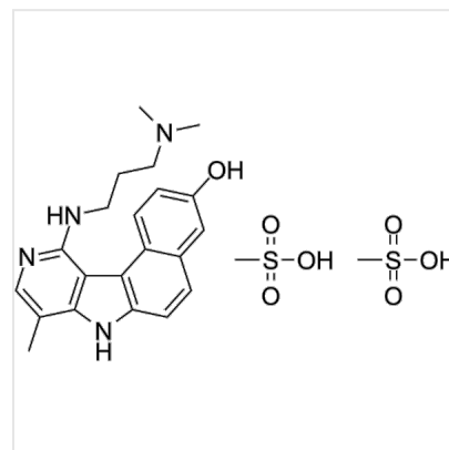
Structure Intopicline dimesylate, CAS 133711-99-6
