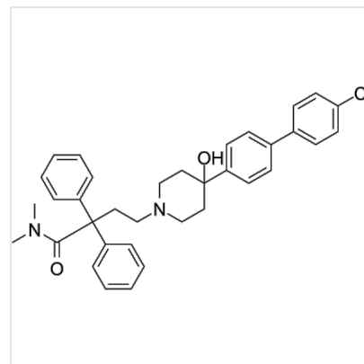
Structure Loperamide phenyl, CAS 1391052-94-0
