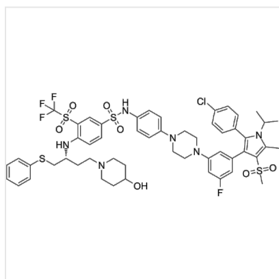
Structure BM-1197, CAS 1391107-89-3
