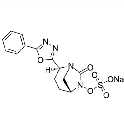
Structure Antibacterial agent 44, CAS 1426572-49-7
