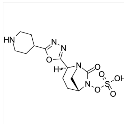
Structure Antibacterial agent 34, CAS 1426572-58-8
