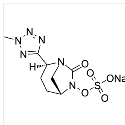
Structure Antibacterial agent 58, CAS 1426572-65-7
