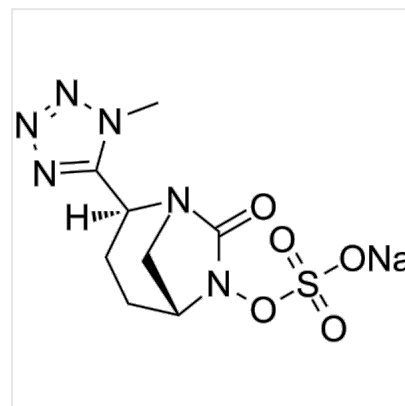
Structure Antibacterial agent 59, CAS 1426572-66-8
