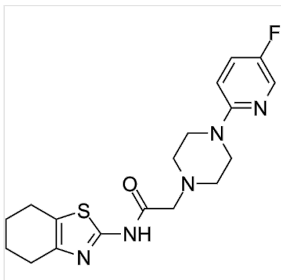
Structure FATP1-IN-1, CAS 1431945-95-7
