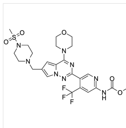
Structure CYH33, CAS 1494684-28-4
