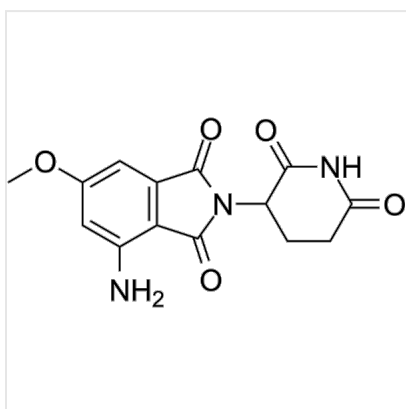
Structure Pomalidomide-6-O-CH 3 , CAS 1547163-08-5
