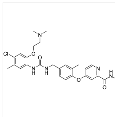
Structure DDR2-IN-1, CAS 1573053-23-2
