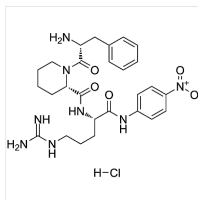
Structure H-D-Phe-Pip-Arg-pNA hydrochloride, CAS 160192-34-7
