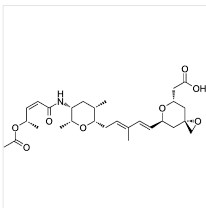
Structure Thailanstatin D, CAS 1609105-89-6
