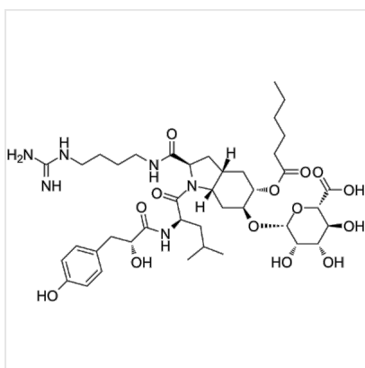
Structure Aeruginosin 865, CAS 1611990-01-2
