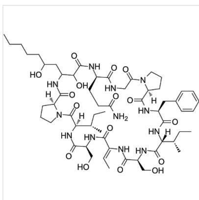
Structure Muscotoxin A, CAS 1653999-47-3
