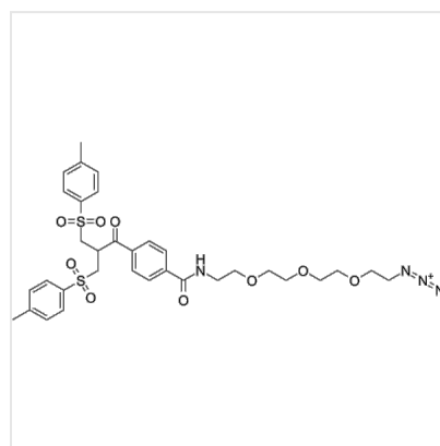
Structure Bis-sulfone-PEG3-Azide, CAS 1802908-01-5
