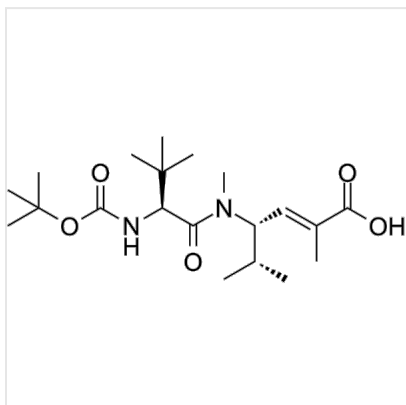
Structure Hemiasterlin derivative-1, CAS 1887046-60-7
