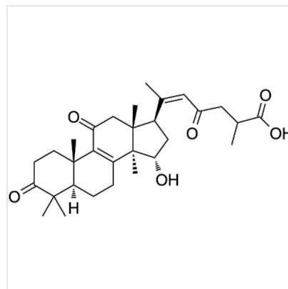
Structure 15a-Hydroxy-3,11,23-trioxo-lanost-8,20-dien-26-oic acid, CAS 1961358-01-9
