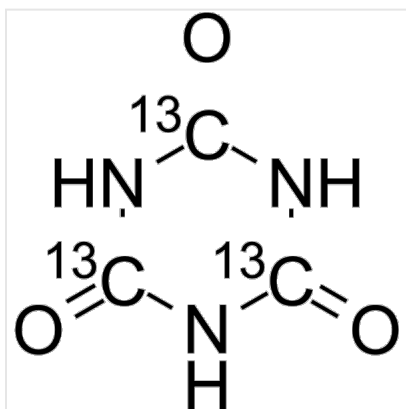
Structure Cyanuric acid-13C3, CAS 201996-37-4
