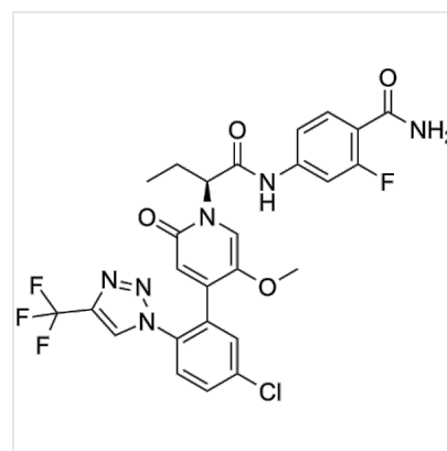
Structure Asundexian, CAS 2064121-65-7
