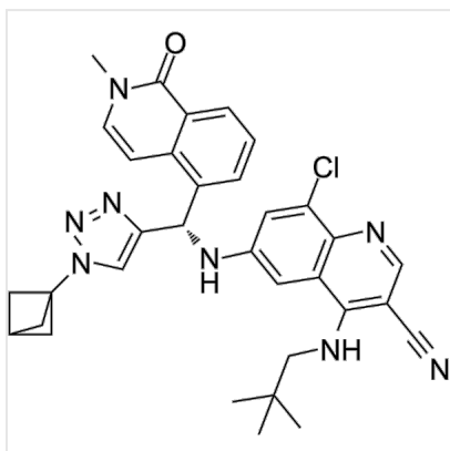
Structure Tilpisetib, CAS 2065153-41-3
