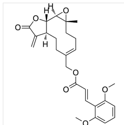
Structure anti-TNBC agent-1, CAS 2289585-58-4
