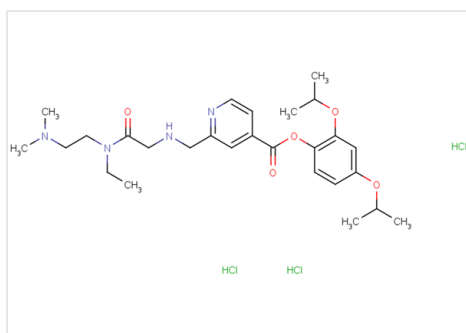
Structure JQKD82 trihydrochloride, CAS T39989L
