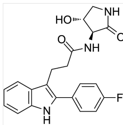
Structure APOL1-IN-1, CAS 2446817-72-5
