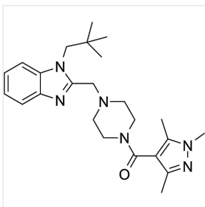
Structure Ftase inhibitor III, CAS 2710375-18-9
