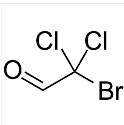
Structure Bromodichloroacetaldehyde, CAS 34619-29-9
