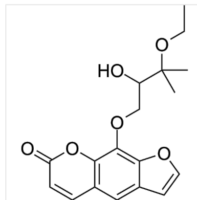
Structure 8-(3-Ethoxy-2-hydroxy-3-methylbutoxy)psoralen, CAS 55481-87-3
