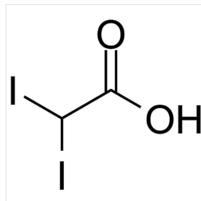
Structure Diiodoacetic acid, CAS 598-89-0
