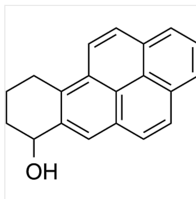
Structure 7,8,9,10-Tetrahydrobenzo[pqr]tetraphen-7-ol, CAS 6272-55-5
