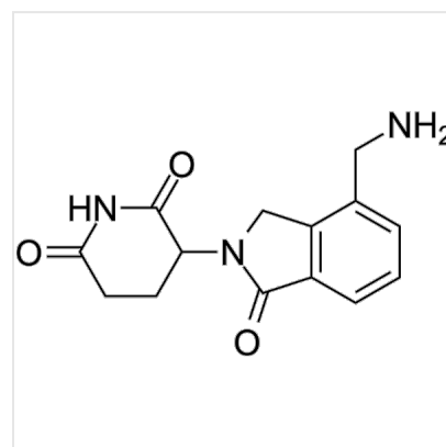
Structure Lenalidomide-4-aminomethyl, CAS 790652-68-5
