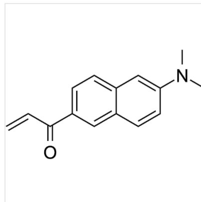
Structure Acrylodan, CAS 86636-92-2
