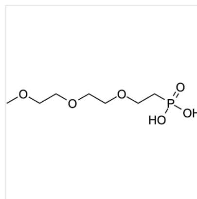
Structure m-PEG3-phosphonic acid, CAS 96962-42-4
