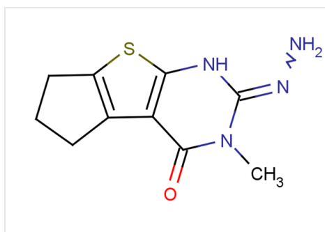
Structure WAY-301207, CAS 351342-00-2
