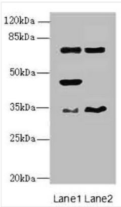
WB (Western Blot) Western blotAll lanes: EHF antibody at 4.95ug/mlLane 1 : Mouse brain tissueLane 2 : Mouse lung tissueSecondaryGoat polyclonal to Rabbit IgG at 1/10000 dilutionPredicted band size: 35,33,38 kDaObserved band size: 35,45,63 kDa
