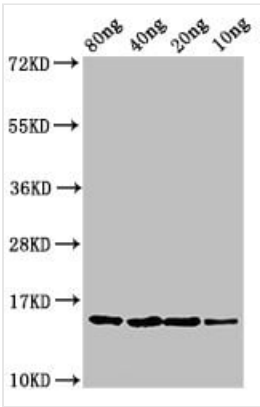
WB (Western Blot) Western BlotPositive WB detected in Recombinant proteinAll lanes: yebF antibody at 2.7ug/mlSecondaryGoat polyclonal to rabbit IgG at 1/50000 dilutionPredicted band size: 15 KDaObserved band size: 15 KDa
