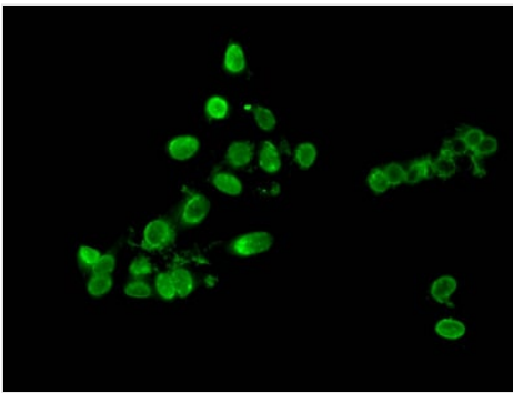
IF (Immunofluorescence) Immunofluorescent analysis of Hela cells using AAA234281 at a dilution of 1:100 and Alexa Fluor 488-conjugated AffiniPure Goat Anti-Rabbit IgG(H+L)
