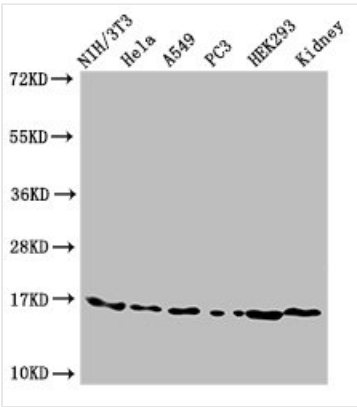
WB (Western Blot) Western BlotPositive WB detected in: NIH/3T3 cell acid extracts, Hela cell acid extracts, A549 cell acid extracts, PC3 cell acid extracts, HEK293 cell acid extracts, Mouse kidney tissueAll lanes: HIST1H3A antibody at 3ug/mlSecondaryGoat polyclonal to rabbit IgG at 1/50000 dilutionPredicted band size: 16 KDaObserved band size: 16 KDa
