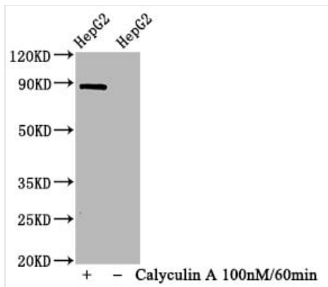
WB (Western Blot) Western BlotPositive WB detected in?HepG2 whole cell lysate(treated with Calyculin A or not)All lanes?Phospho-STAT1 antibody at 1.065ug/mlSecondaryGoat polyclonal to rabbit IgG at 1/50000 dilutionPredicted band size: 87 KDaObserved band size: 87 KDa
