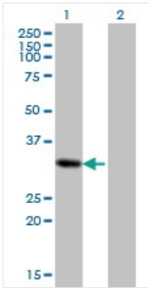
WB (Western Blot) Western Blot analysis of IRF2 expression in Hela NE using.
