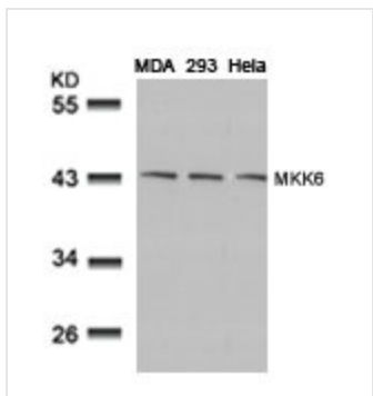
WB (Western Blot) Western blot analysis of extracts from MDA, 293 and Hela cells using MKK6(Ab-207) Antibody.
