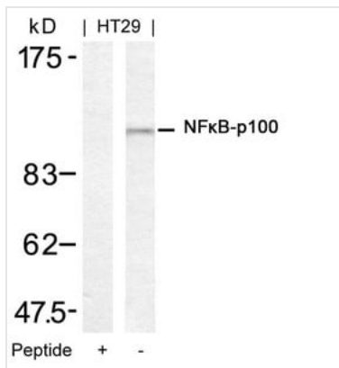
WB (Western Blot) Western blot analysis of extracts from HT29 cells using NFkB-p100(Ab-872) Antibody and the same antibody preincubated with blocking peptide.
