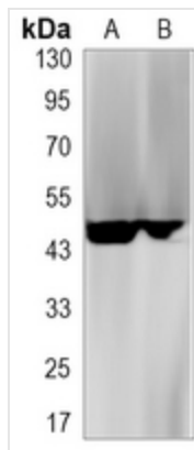
WB (Western Blot) Western blot analysis of CD95 expression in HeLa (A), Jurkat (B) whole cell lysates. (Predicted band size: 38 kD; Observed band size: 40-50 kD)
