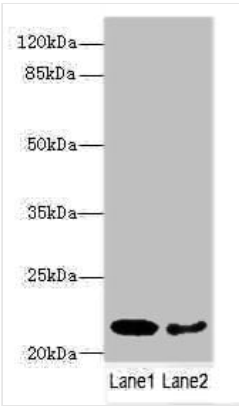
WB (Western Blot) Western blotAll lanes: PRDX2 antibody at 9ug/mlLane 1: Mouse liver tissueLane 2: Mouse spleen tissueSecondaryGoat polyclonal to rabbit IgG at 1/10000 dilutionPredicted band size: 22,16 kDaObserved band size: 22 kDa
