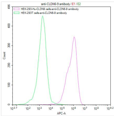
FCM/FACS (Flow Cytometry) Untransfected HEK-293T cells (green line) and transfected Human CLDN9 HEK-293T stable cells (red line) were stained with anti-CLDN6/9 antibody (AAA279305) (2ug/1*106cells), washed and then followed by APC-conjugated anti-Mouse IgG Fc antibody and analyzed with flow cytometry.
