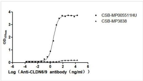
ELISA The Binding Activity of Human CLDN6 with Anti-CLDN6-9 recombinant antibodyActivity: Measured by its binding ability in a functional ELISA. Immobilized Human CLDN6-9 (CSB-MP005511HU) at 10 ug/mL can bind Anti-CLDN6-9 recombinant antibody. The EC50 is 2.876-3.657 ng/mL. The VLPs (CSB-MP3838) is negative control.
