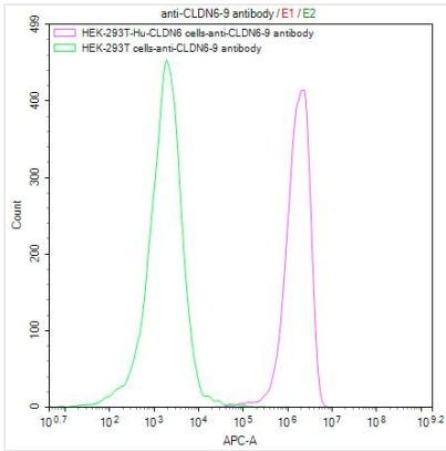
FCM/FACS (Flow Cytometry) Untransfected HEK-293T cells (green line) and transfected Human CLDN6 HEK-293T stable cells (red line) were stained with anti-CLDN6/9 antibody(AAA279305) (2ug/1*106cells), washed and then followed by APC-conjugated anti-Mouse IgG Fc antibody and analyzed with flow cytometry.
