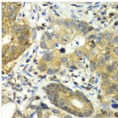
IHC (Immunohistochemisry) Immunohistochemistry of paraffin-embedded human gastric cancer using DPP3 antibody at dilution of 1:100 (40x lens).
