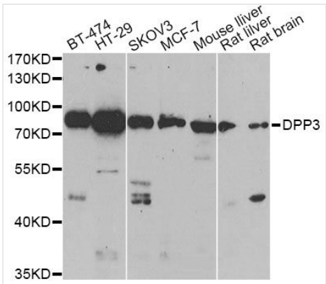
WB (Western Blot) Western blot analysis of extracts of various cell lines, using DPP3 antibody at 1:1000 dilution.Secondary antibody: HRP Goat Anti-Rabbit IgG (H+L) at 1:10000 dilution.Lysates/proteins: 25ug per lane.Blocking buffer: 3% nonfat dry milk in TBST.Detection: ECL Basic Kit.Exposure time: 90s.
