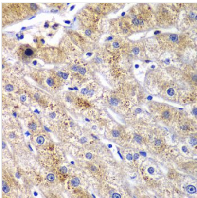
IHC (Immunohiostchemistry) Immunohistochemistry of paraffin-embedded human liver injury using DPP3 antibody at dilution of 1:100 (40x lens).
