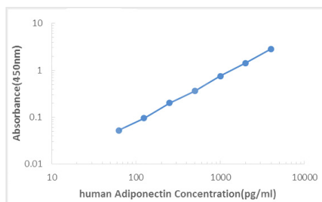
Standard Curve (Sample) Human Adiponectin ELISA Kit
