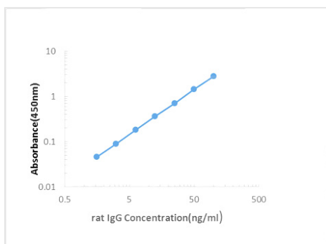
Standard Curve (Sample) Rat IgG ELISA Kit
