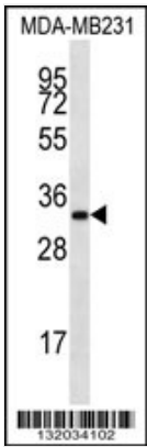
WB (Western Blot) LIX1L Antibody (Center) western blot analysis in MDA-MB231 cell line lysates (35ug/lane). This demonstrates the LIX1L antibody detected the LIX1L protein (arrow).
