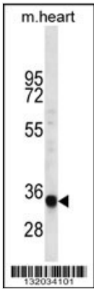
WB (Western Blot) LIX1L Antibody (Center) western blot analysis in mouse heart tissue lysates (35ug/lane). This demonstrates the LIX1L antibody detected the LIX1L protein (arrow).
