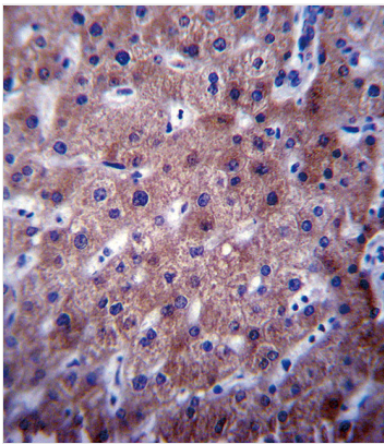
IHC (Immunohistochemistry) CYP2C19 Antibody (Center) immunohistochemistry analysis in formalin fixed and paraffin embedded human liver tissue followed by peroxidase conjugation of the secondary antibody and DAB staining. This data demonstrates the use of CYP2C19 Antibody (Center) for immunohistochemistry. Clinical relevance has not been evaluated.
