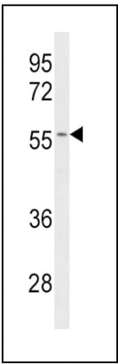
WB (Western Blot) Western blot analysis of CYP2C19 Antibody (Center) in Jurkat cell line lysates (35ug/lane). CYP2C19 (arrow) was detected using the purified Pab.
